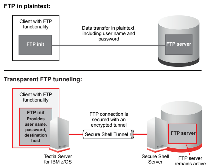
Figure 5.3. Transparent FTP tunneling
