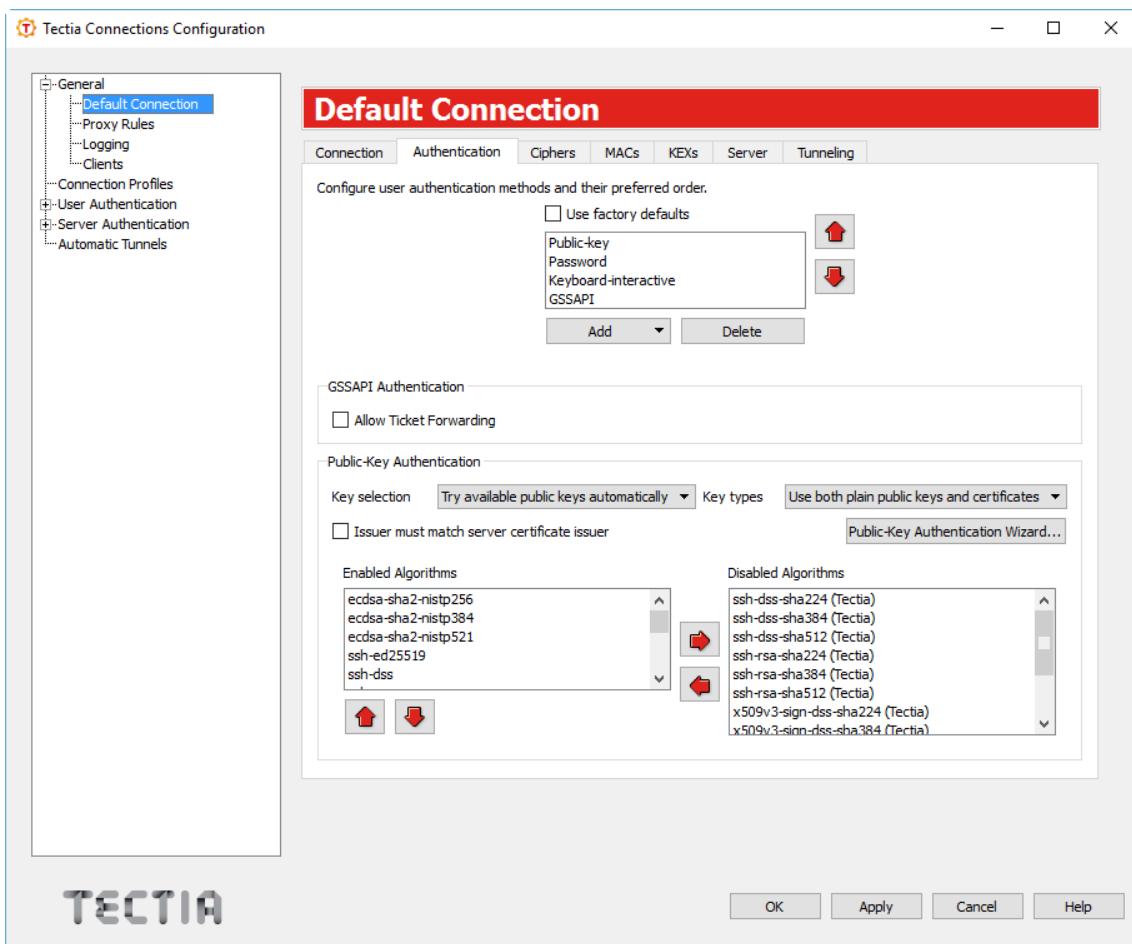
Figure A.5. Authentication methods for Tectia Client
