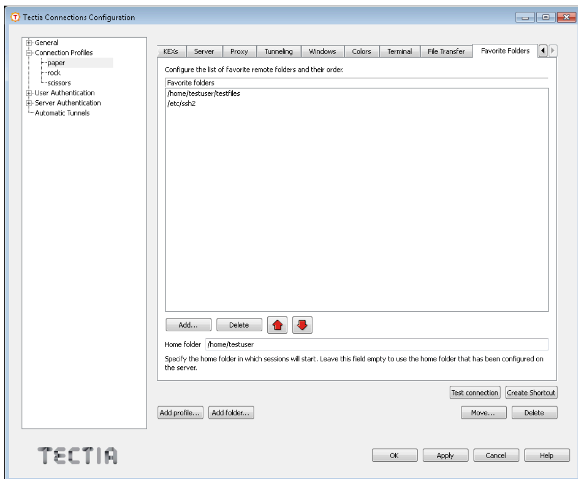
Figure A.33. Defining favorite remote folders for file transfer
