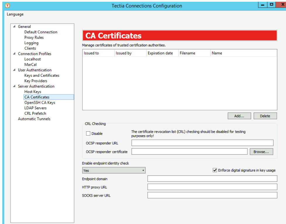
Figure A.39. Defining CA certificates
