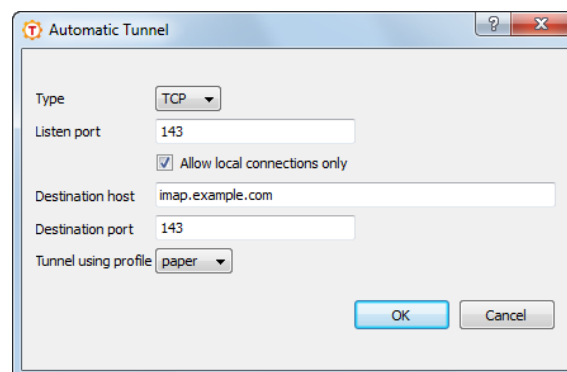
Figure A.45. Adding a new automatic tunnel
