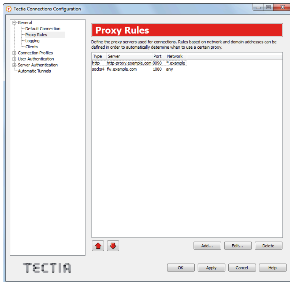
Figure A.11. Defining proxy rules
