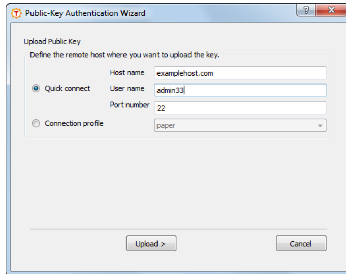
Figure A.18. Uploading a key
