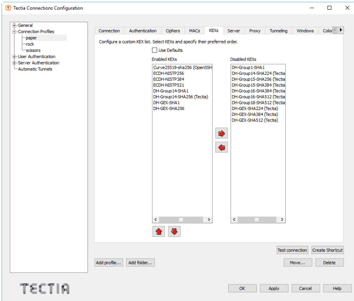
Figure A.21. Defining a KEX list for the profile
