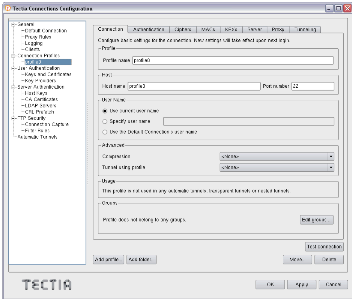
Figure A.1. Connection profile tabs on Linux
