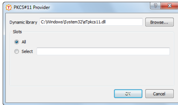
Figure A.36. Defining a PKCS #11 provider, Aladdin eToken DLL path shown as an example
