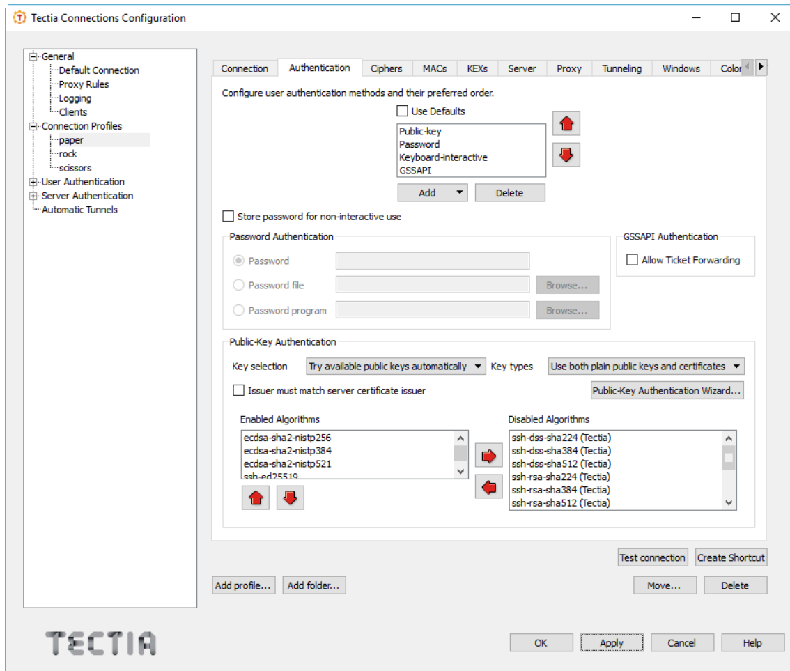
Figure A.16. Configuring authentication methods for the profile
