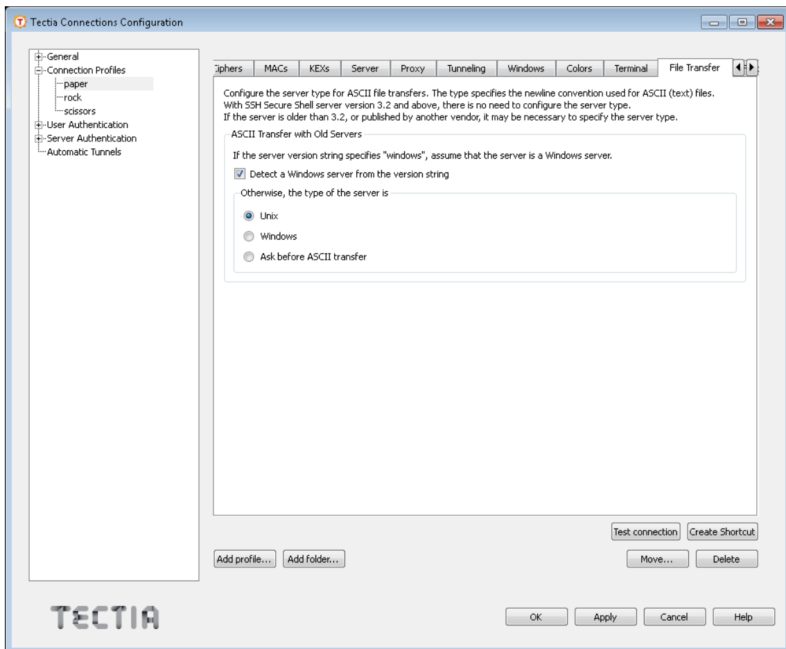
Figure A.32. Defining Tectia file transfer settings
