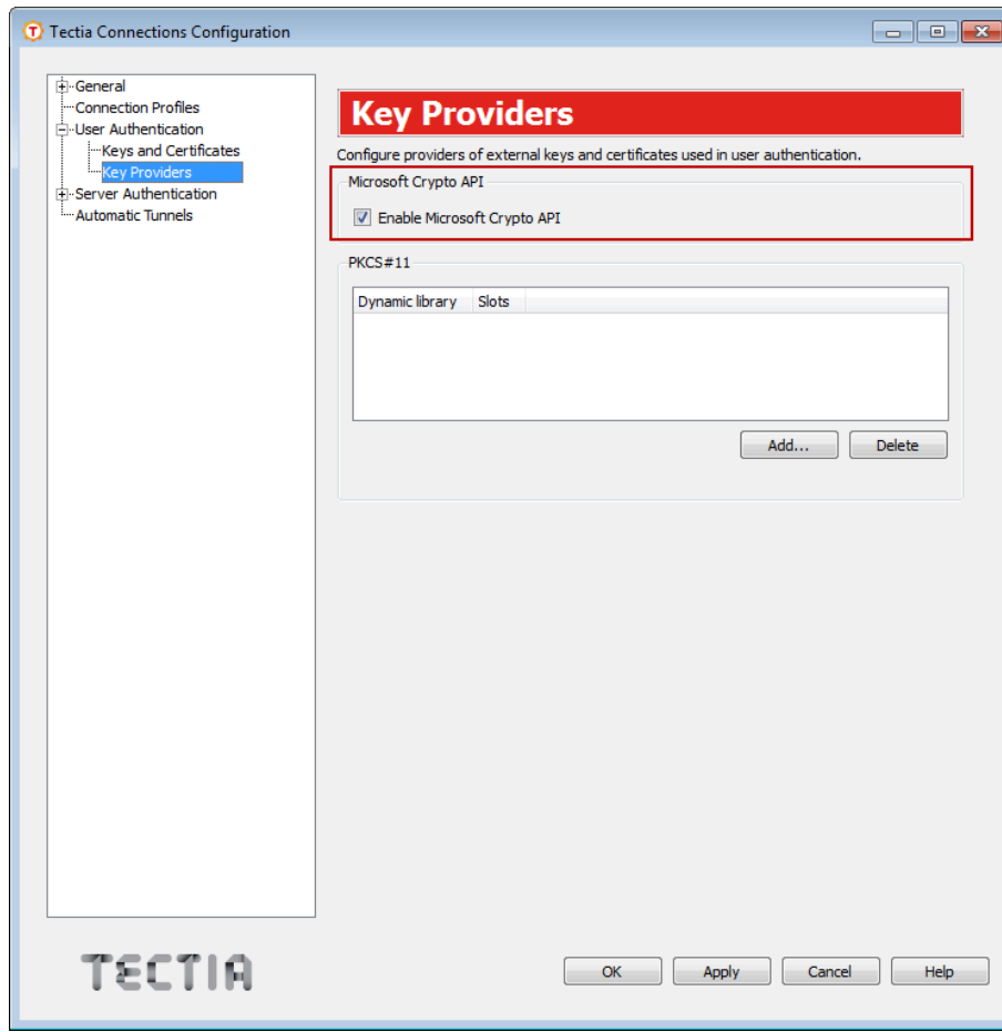
Figure 4.8. Enabling Microsoft Crypto API as a certificate provider
