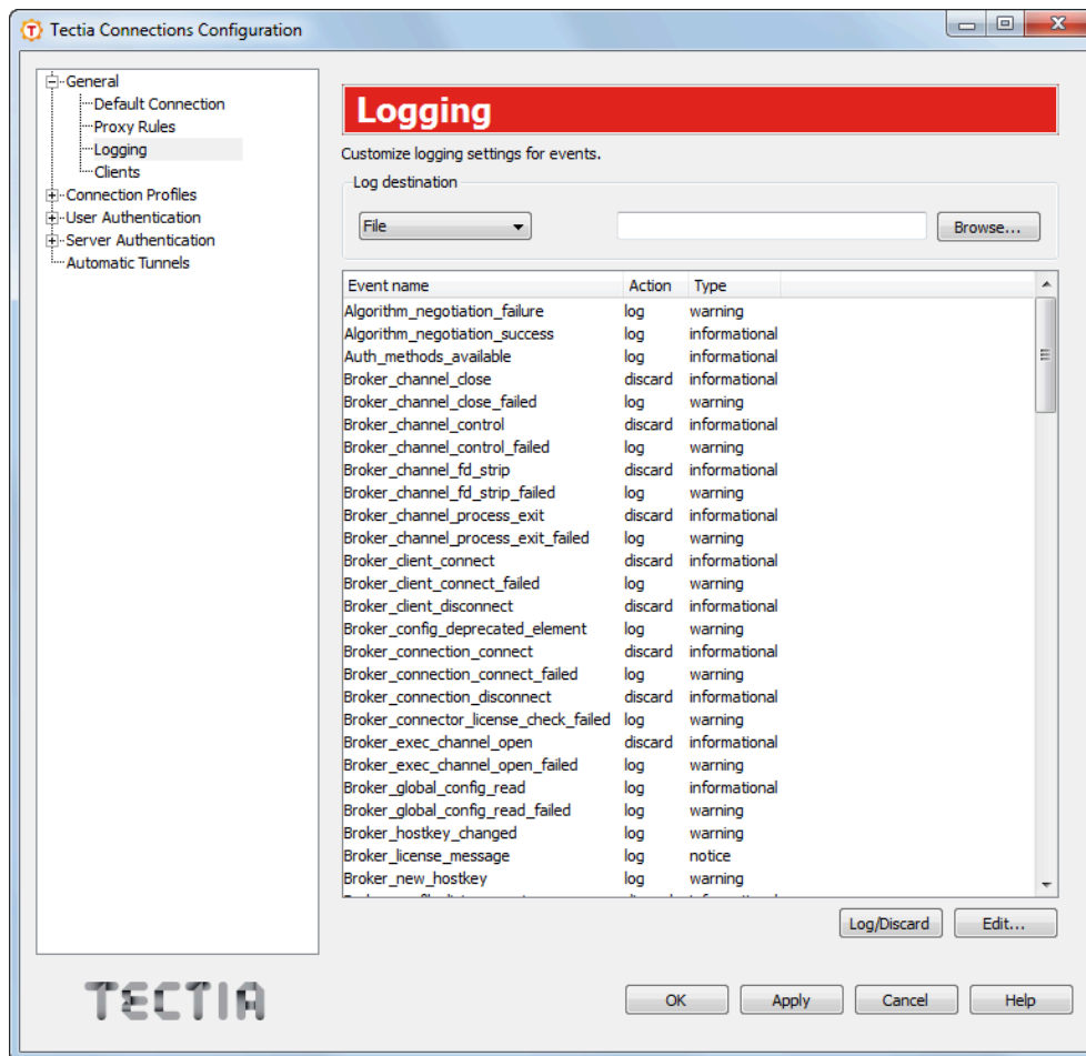
Figure A.13. Logging settings
