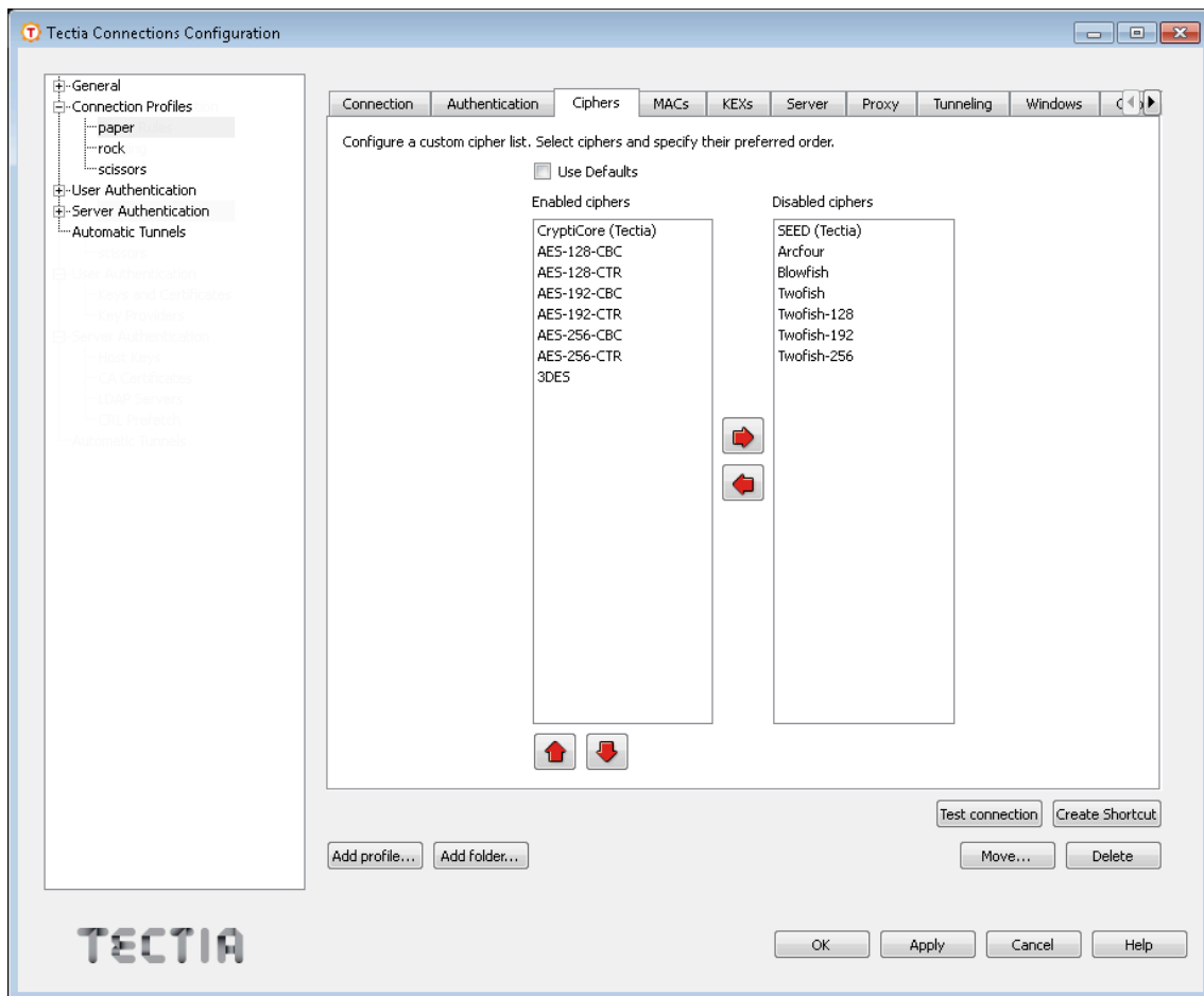
Figure A.19. Defining a cipher list for the profile
