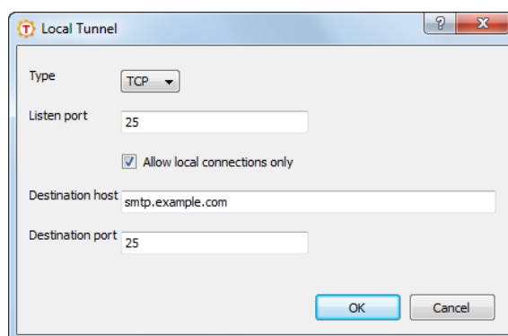
Figure A.26. Defining a local tunnel
