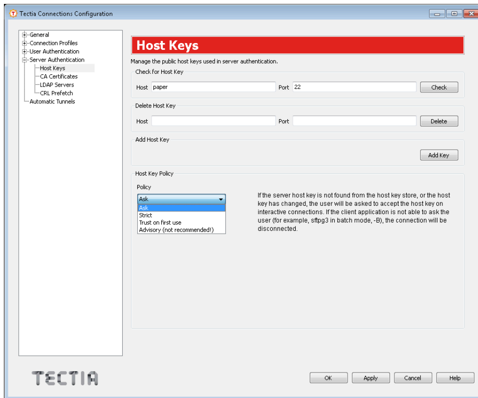
Figure A.37. Defining server host keys settings
