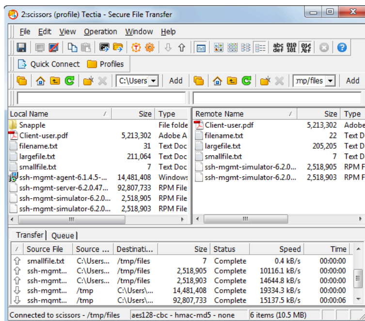
Figure 5.1. Tectia Secure File Transfer GUI
