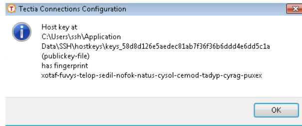
Figure A.38. Server public host key information
