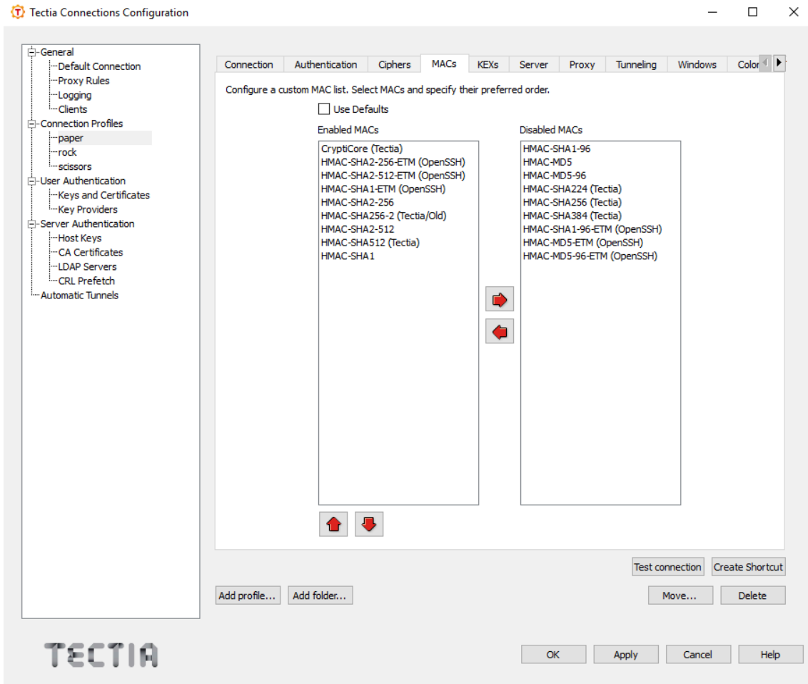
Figure A.20. Defining a MAC list for the profile
