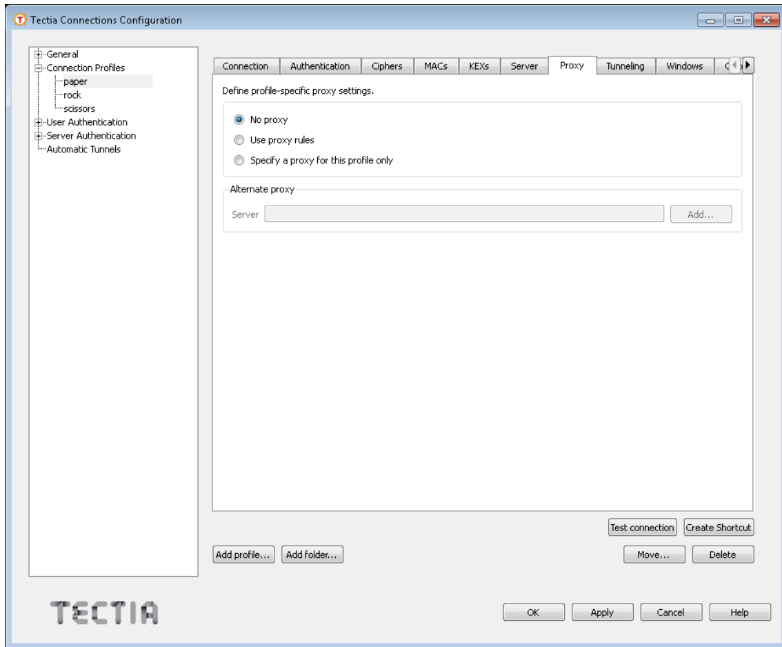
Figure A.23. Defining proxy settings for the profile
