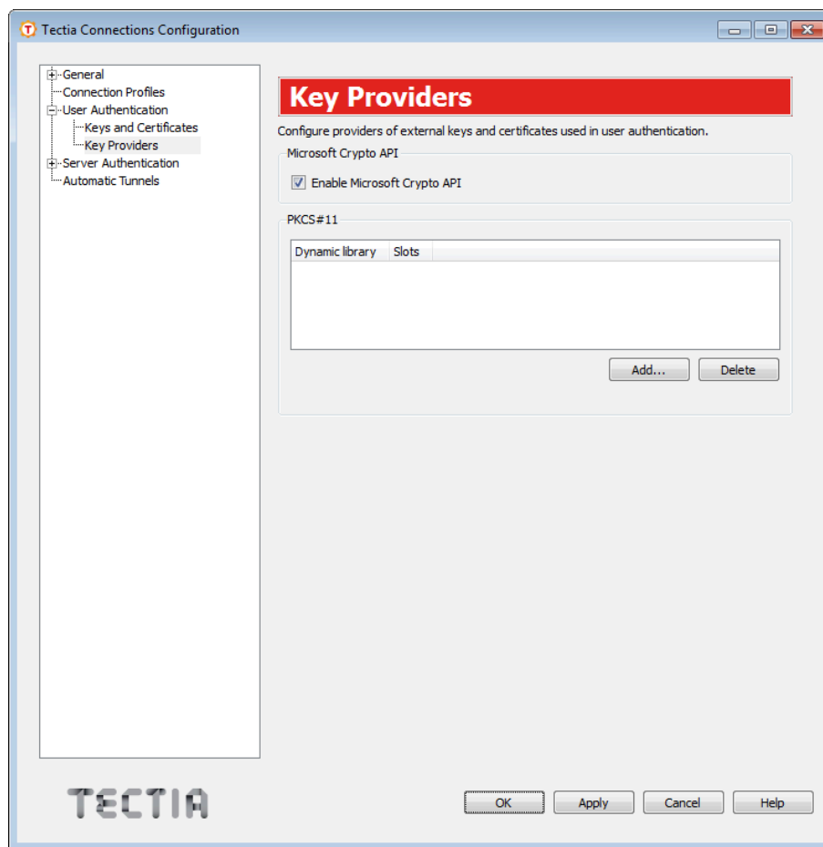
Figure A.35. Defining key providers
