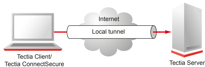
Figure 6.2. Simple local tunnel
