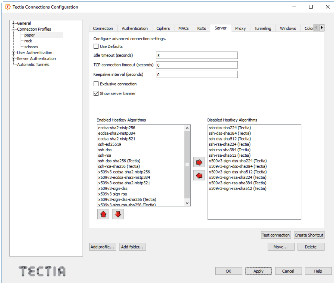
Figure A.22. Defining server connection settings for the profile
