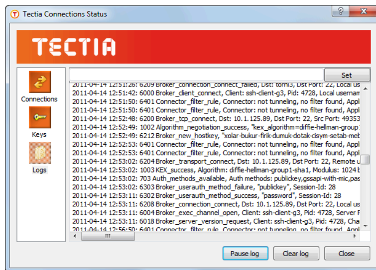
Figure A.49. The Logs view of the Status window
