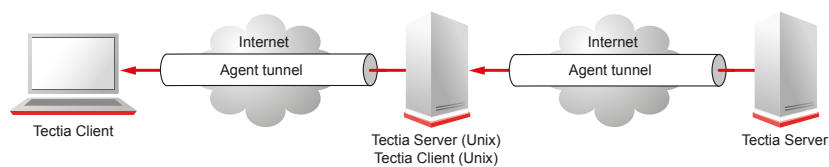
Figure 6.7. Agent forwarding
