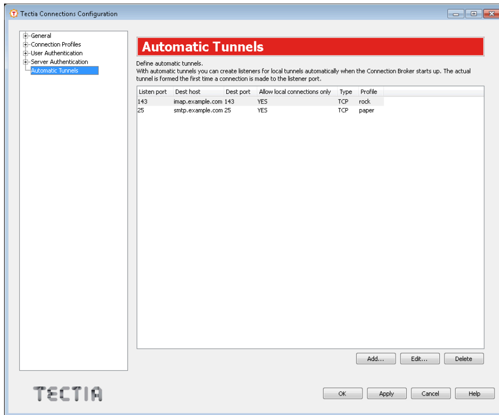
Figure A.44. Defining automatic tunnels
