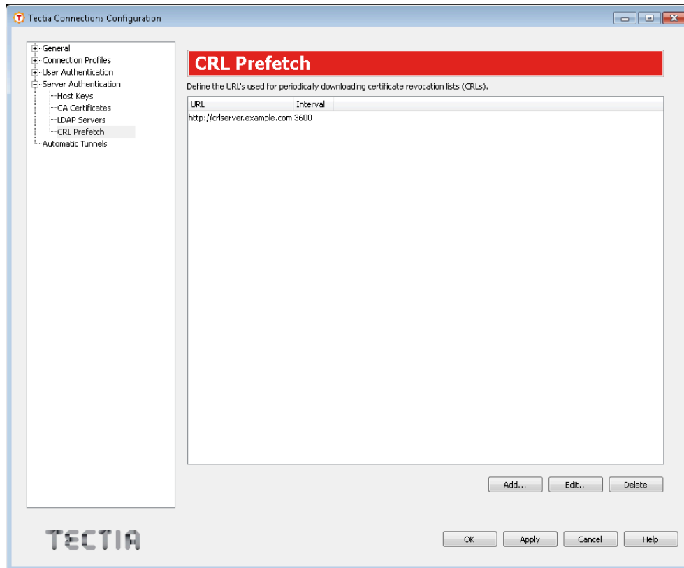
Figure A.42. Defining CRL prefetch settings
