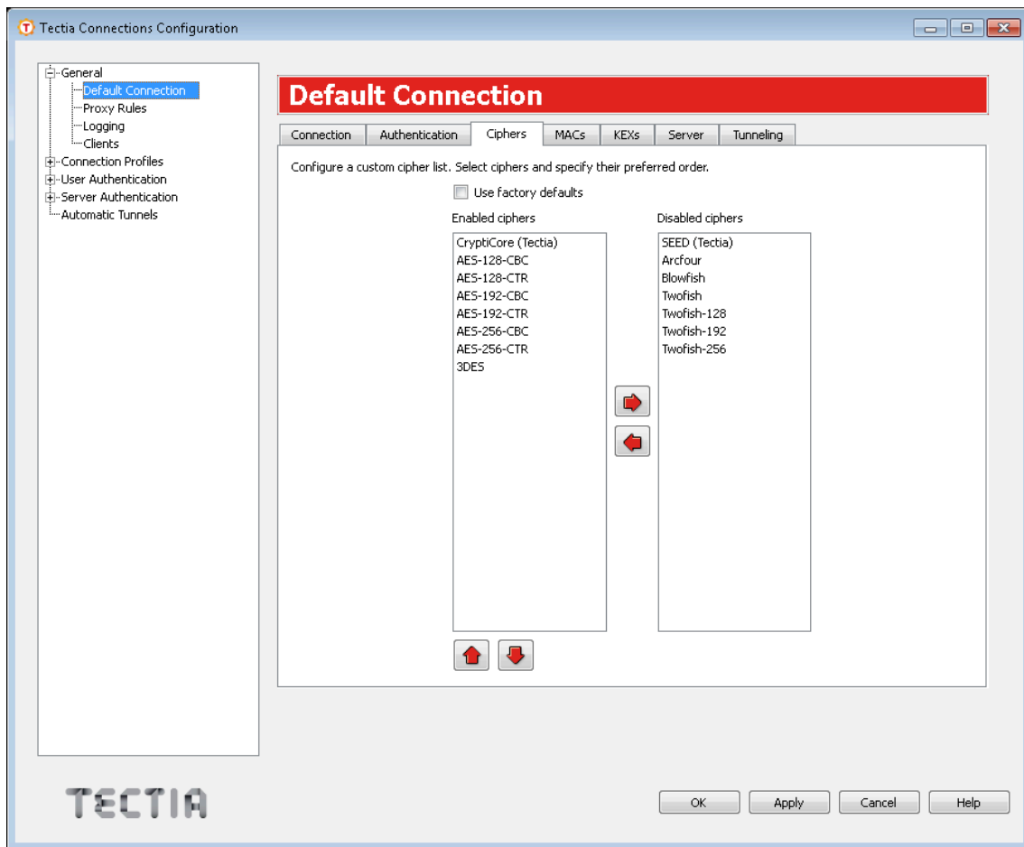
Figure A.6. Defining a cipher list
